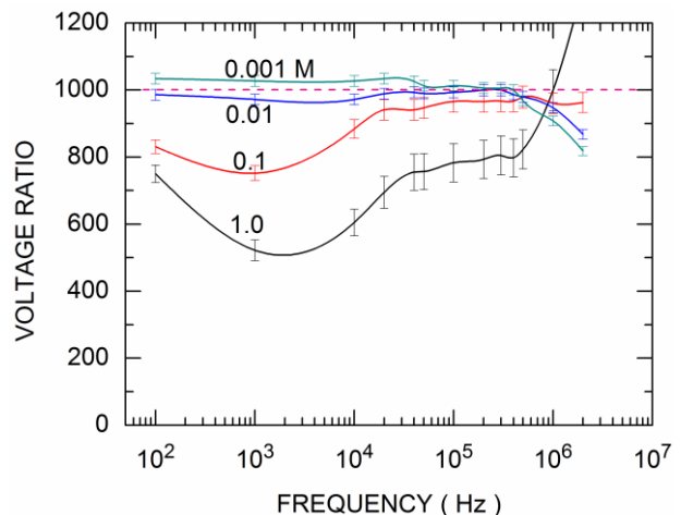
Fig.2 – Voltage ratio for 1000X voltage divider for each molar concentration of \text{MgSO}_4 .
